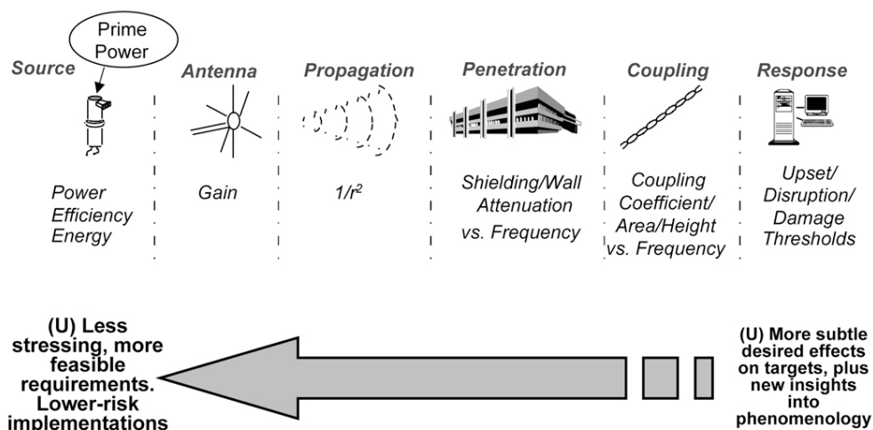
Figure 12. Source-to-Target Response
