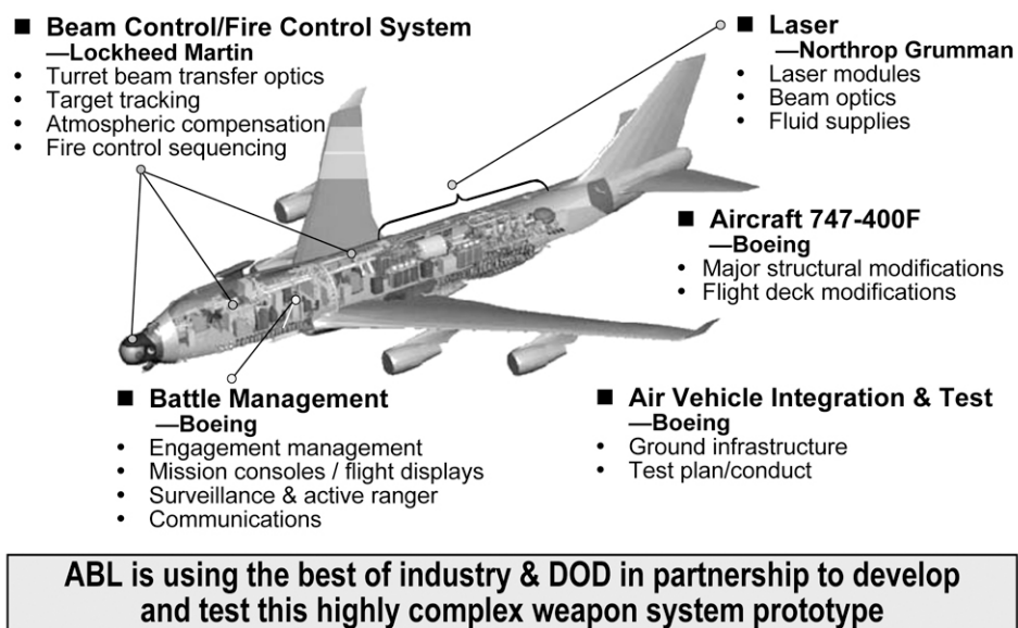
Figure 1. Airborne Laser Weapon System Elements
