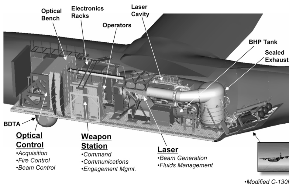
Figure 4. High Power A/C Configuration
